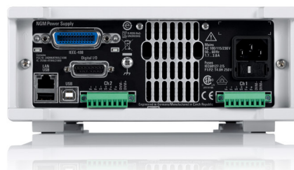
R&S®NGM202, rear view
